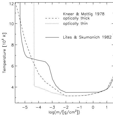
Fig. 2. Run of temperature with column mass density m for various umbra models.
