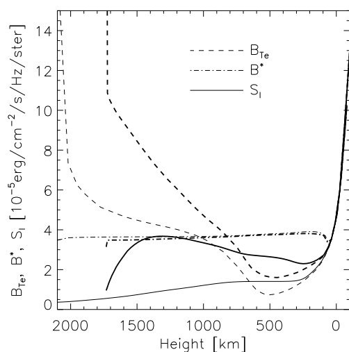
Fig. 7. Height dependence of Planck function for electron temperature, B_{Te} , radiative term B^* in Eq. 4, and line source function S_l ; thin: VAL C model (Vernazza et al. 1981); thick: FAL P model (Fontenla et al. 1993).
