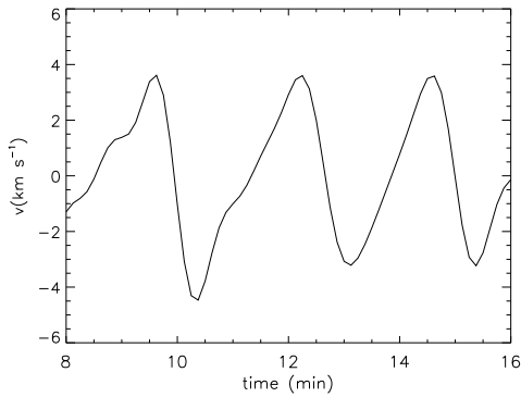
Fig. 4. Detail of velocity time sequence in a sunspot umbra measured in He I 10830 Å showing sawtooth-shaped evolution; from Felipe et al. (2008).
