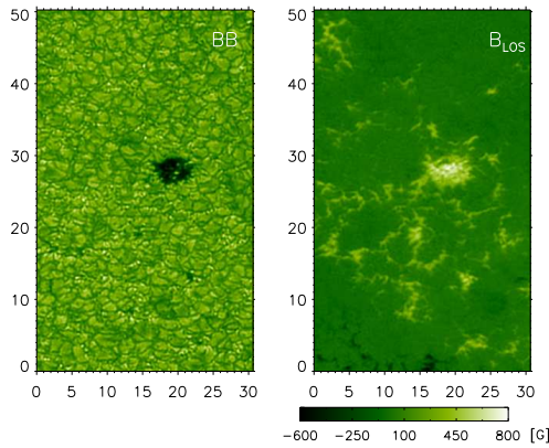
Fig. 5. Weak plage with pore. Left: broadband in 630 nm; right: LOS component of magnetic field; distance of tick marks in arcsec; from Bello González & Kneer (2008).
