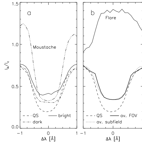
Fig. 10. Several H\alpha profiles from active region compared with quiet-Sun profile (QS) from an area nearby. Profiles denoted as ‘bright’ and ‘dark’ are temporal and 0'.33 \times 0'.33 averages from the areas ‘bright’ and ‘dark’ in Fig 9, respectively. ‘Av. subfield’ and ‘av. FOV’ denote the average profile from region ‘A’ and from the whole field-of-view (FOV) in the same figure, respectively.
