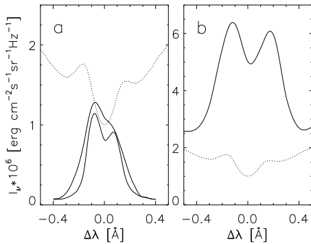
Fig. 1. Central part of Ca II K line. (a): quiet Sun (dotted) from Fourier Transform Spectrometer Atlas (Brault & Neckel, quoted by Neckel 1999), from sunspot umbra (thin solid) and from model (thick solid), latter two after Lites & Skumanich (1982). The model profile is convolved with a Gaussian corresponding to a ‘macro-turbulence’ of 5 \text{ km s}^{-1} . (b): quiet-Sun K line (dotted) and from a plage (after Shine & Linsky 1972). Note the different scales in panels (a) and (b).
