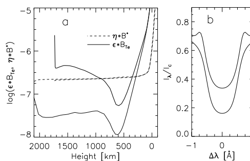
Fig. 8. (a): Terms \varepsilon \cdot B_{Te} and \eta \cdot B^* in Eq. 4 in units of \text{erg cm}^{-2} \text{s}^{-1} \text{Hz}^{-1} \text{ster}^{-1} as functions of height; thin: VAL C model, thick: FAL P model. (b): resulting H\alpha profiles.
