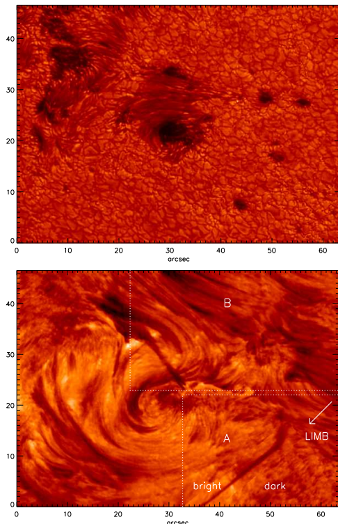
Fig. 9. Section of active region AR 10875 in broadband around 630 nm (upper) and in H\alpha +0.5 \text{ \AA} off line centre (lower), from Sánchez-Andrade Nuño et al. (2008).
