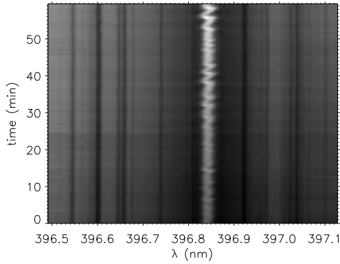
Fig. 3. Temporal evolution of Ca II H in a sunspot umbra; from Felipe et al. (2008).
