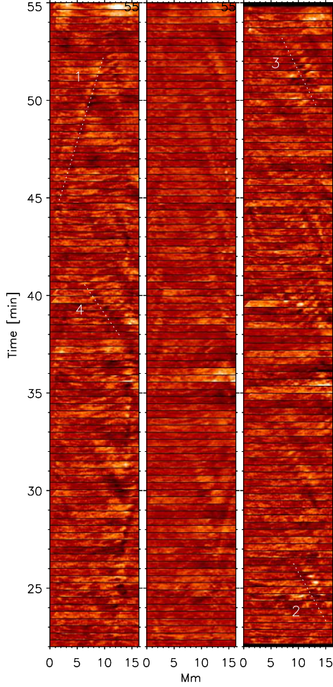
Fig. 13. Space-time slices (16.2 Mm \times 0.8 Mm, \Delta t = 22 s, after high-pass filtering) from fibrils in region ‘B’ of Fig. 9; from left to right: LOS velocity, H \alpha line centre intensity, and differences I_{0.5}(t_{i+1}) - I_{0.5}(t_i) , I_{0.5} = intensity at +0.5 Å off line centre.
